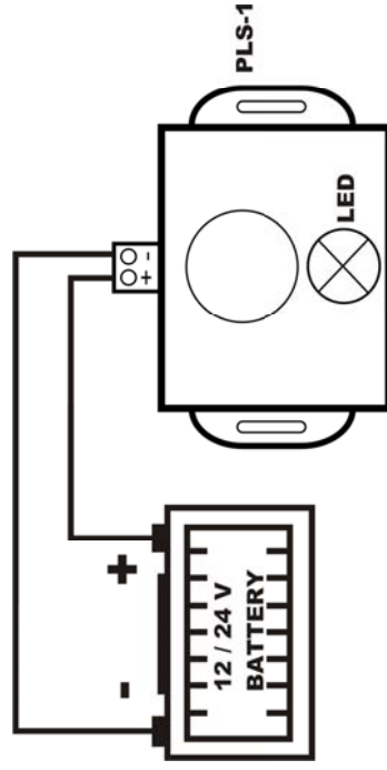
2: Connection schematic.
